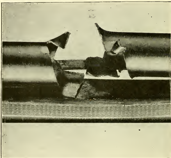
Barrel burst towards the Muzzle by Nitro-Powder.
